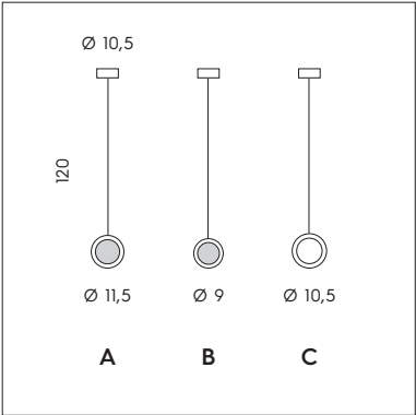
SP 7/330 A - B - C 6W STRIP LED 800 lumen - 3000K CE IP20
