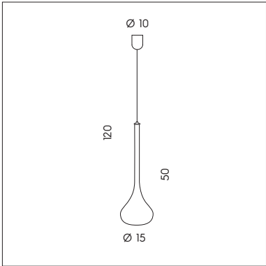
SP 7/294 D-50 1 x max 6W GU10 LED CE
