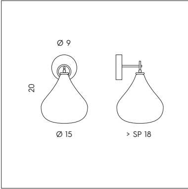
LP 6/294 1 x max 6W GU10 LED CE
