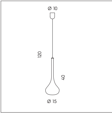
SP 7/294 C-40 1 x max 6W GU10 LED CE
