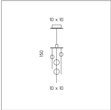
SP 7/236 1 x max 5W G9 LED CE
