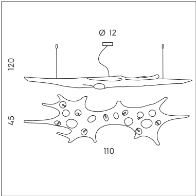
SP 1057/110S 14 x max 2W G4 LED CE
