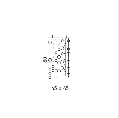
SP H/236 8 x max 5W G9 LED CE
