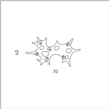
LP 1057/40 6 x max 2W G4 LED CE
