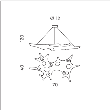
SP 1057/70S 8 x max 2W G4 LED CE
