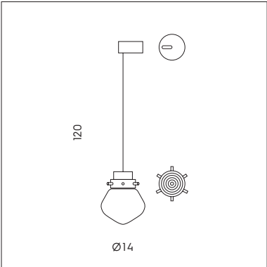
SP 7/295 1 x 6W LED 768 lumen 3000K CE IP20
