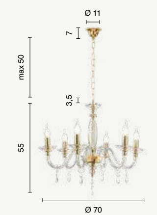
lampadario chandelier LP.FIAMMA/6 power: 6 x E14 voltage: 220-230V
