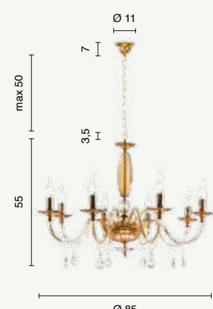
lampadario chandelier LP.CECILIA/8-ORO LP.CECILIA/8A LP.CECILIA/8-TORT power: 8 x E14 voltage: 220-230V
