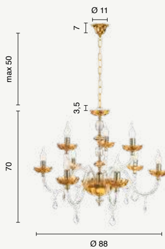
lampadario chandelier LP.PATRICIA/9A power: 9 x E14 voltage: 220-230V
