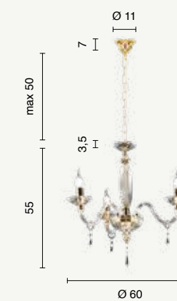
lampadario chandelier LP.FIAMMA/3 power: 3 x E14 voltage: 220-230V
