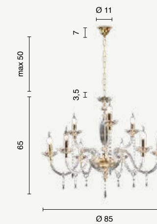
lampadario chandelier LP.FIAMMA/9 power: 9 x E14 voltage: 220-230V
