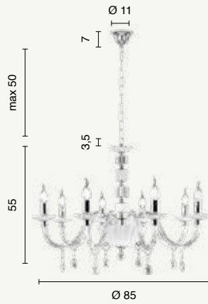
lampadario chandelier LP.LIVIA/8BL LP.LIVIA/8-TOR LP.LIVIA/8-FUME LP.LIVIA/8-OTT power: 8 x E14 voltage: 220-230V
