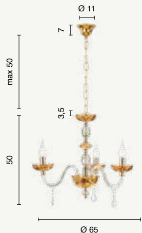
lampadario chandelier LP.PATRICIA/3A power: 3 x E14 voltage: 220-230V
