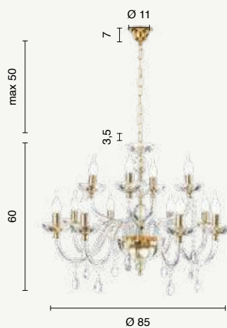
lampadario chandelier LP.BRIGIDA/12 power: 12 x E14 voltage: 220-230V
