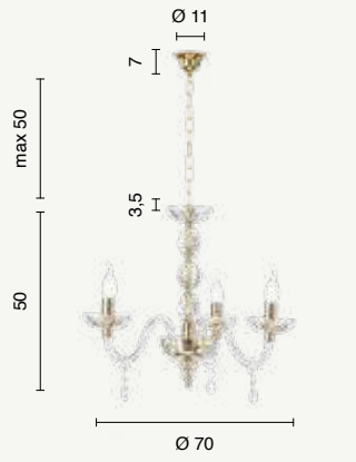
lampadario chandelier LP.BRIGIDA/3 power: 3 x E14 voltage: 220-230V
