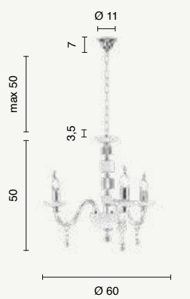
lampadario chandelier LP.LIVIA/3BL LP.LIVIA/3-TOR LP.LIVIA/3-FUME LP.LIVIA/3-OTT power: 3 x E14 voltage: 220-230V
