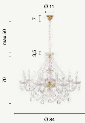
lampadario chandelier LP.OPERA/8 LP.OPERA/8-FUMÈ LP.OPERA/8-TORT power: 8 x E14 voltage: 220-230V
