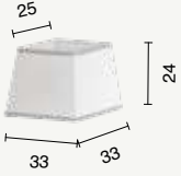
paralume lampshade TC.4018D33 TC.4018D33 TC.4018D33 TC.4018D33
