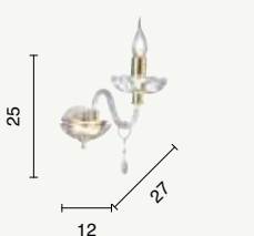
applique wall lamp AP.BRIGIDA/1 power: 1 x E14 voltage: 220-230V
