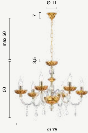
lampadario chandelier LP.PATRICIA/6A power: 6 x E14 voltage: 220-230V
