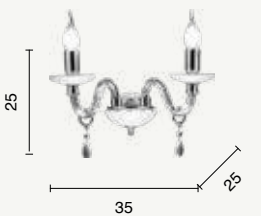
applique wall lamp AP.LIVIA/2BL AP.LIVIA/2-TOR AP.LIVIA/2-FUME AP.LIVIA/2-OTT power: 2 x E14 voltage: 220-230V
