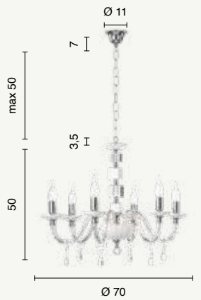
lampadario chandelier LP.LIVIA/6BL LP.LIVIA/6-TOR LP.LIVIA/6-FUME LP.LIVIA/6-OTT power: 6 x E14 voltage: 220-230V
