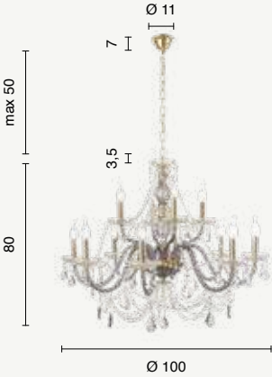
lampadario chandelier LP.OPERA/12 LP.OPERA/12-FUMÈ LP.OPERA/12-TORT power: 12 x E14 voltage: 220-230V
