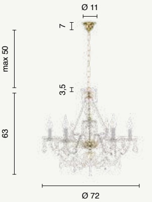
lampadario chandelier LP.OPERA/6 LP.OPERA/6-FUMÈ LP.OPERA/6-TORT power: 6 x E14 voltage: 220-230V
