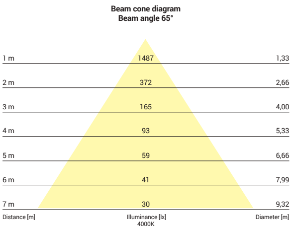
8770, 30W, 4000K, beam angle 65°
