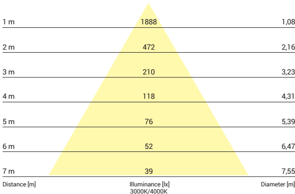
Beam cone diagram Beam angle 60°
