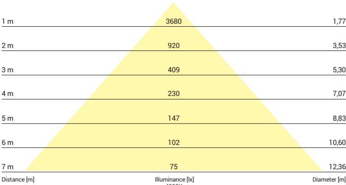
8261, 40W, 4000K, beam angle 83°
