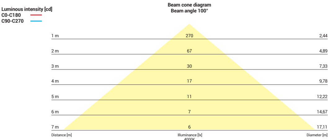
8781, 8W, 4000K, beam angle 100°
