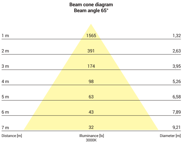
8771, 30W, 3000K, beam angle 65°
