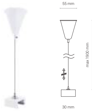
CTLS SUSPENSION KIT
