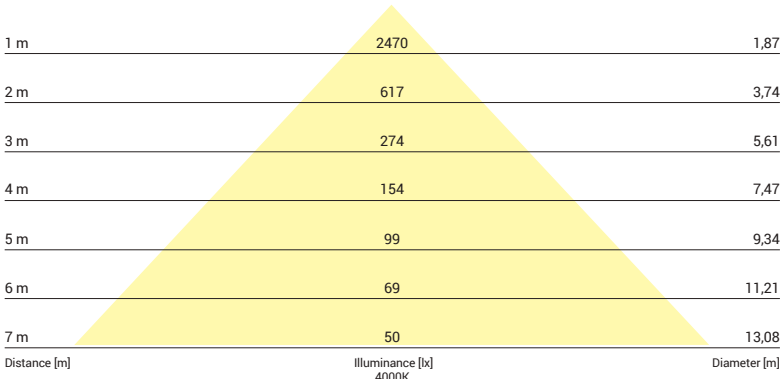
Beam cone diagram Beam angle 86°
