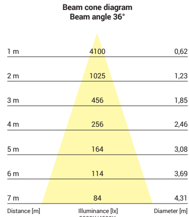
8754, 8755, 8756, 8757, 25W, 3000K, 4000K, beam angle 36°
