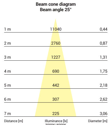
8750, 8751, 8752, 8753, 30W, 3000K, 4000K, beam angle 25°
