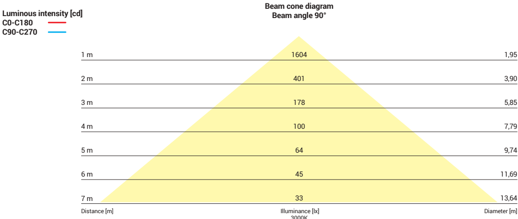
8298, 31W, 3000K, beam angle 90°
