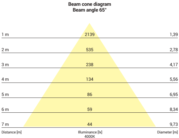
8767, 40W, 4000K, beam angle 65°
