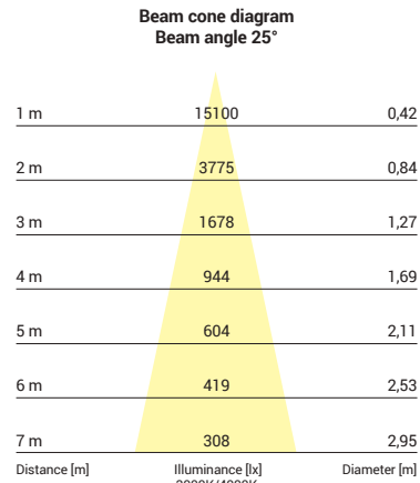
8745, 8746, 8747, 8748, 40W, 3000K, 4000K, beam angle 25°
