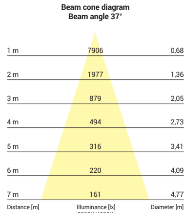
8745, 8746, 8747, 8748, 40W, 3000K, 4000K, beam angle 37°
