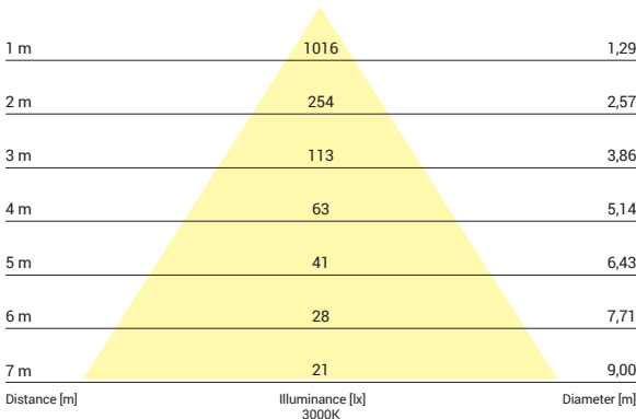
8773, 20W, 3000K, beam angle 65°
