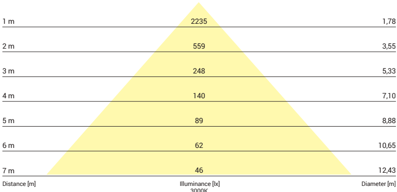
Beam cone diagram Beam angle 83°
