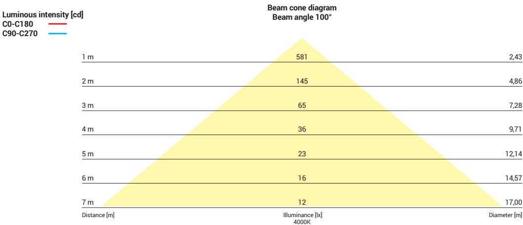
8776, 16W, 4000K, beam angle 100°
