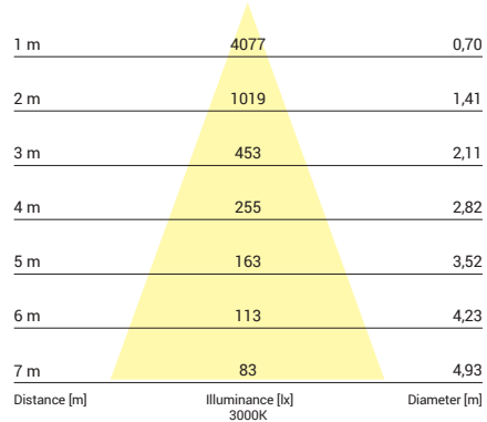
8720, 30W, 3000K, beam angle 40°
