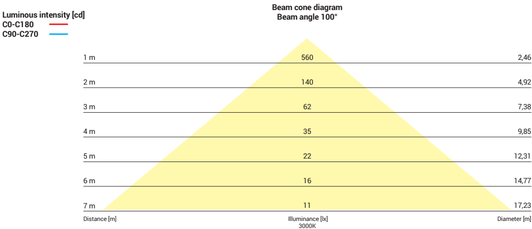
8777, 16W, 3000K, beam angle 100°
