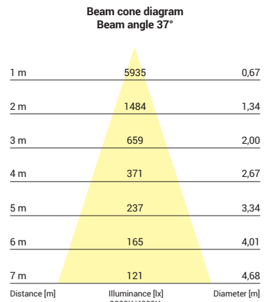
8750, 8751, 8752, 8753, 30W, 3000K, 4000K, beam angle 37°
