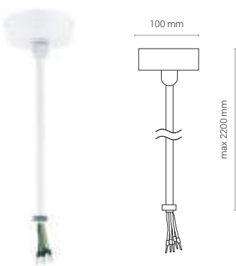
CTLS POWER SUPPLY KIT
