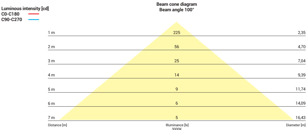
8782, 8W, 3000K, beam angle 100°
