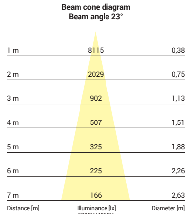
8754, 8755, 8756, 8757, 25W, 3000K, 4000K, beam angle 23°
