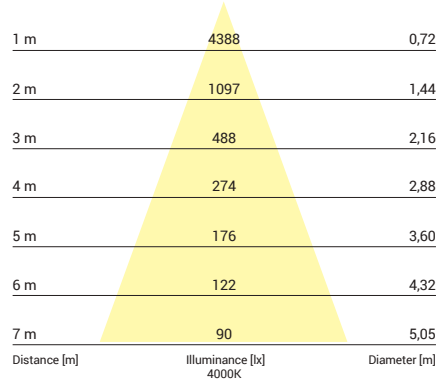
8718, 30W, 4000K, beam angle 40°
