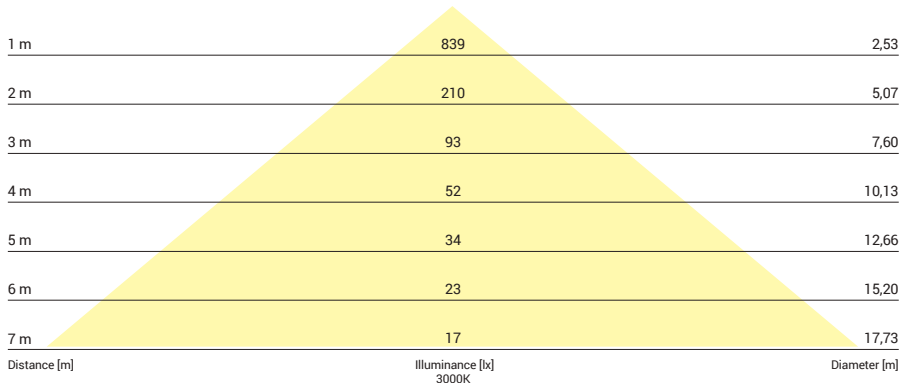
Beam cone diagram Beam angle 100°
