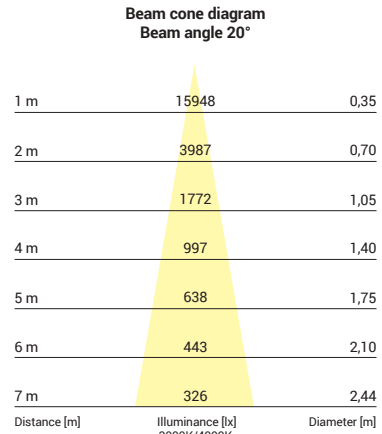
8750, 8751, 8752, 8753, 30W, 3000K, 4000K, beam angle 20°
