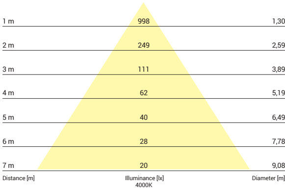
8772, 20W, 4000K, beam angle 65°
