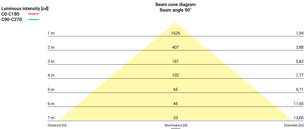
8297, 31W, 4000K, beam angle 90°
