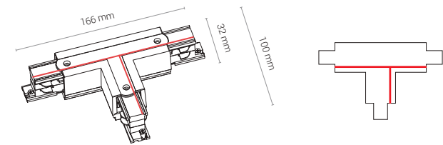
CTLS POWER T CONNECTOR, LEFT 2 (T-L2)
