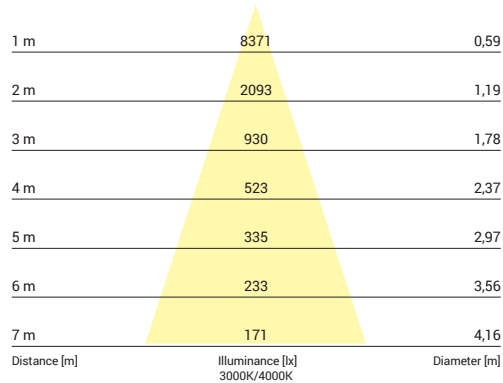
Beam cone diagram Beam angle 36°
