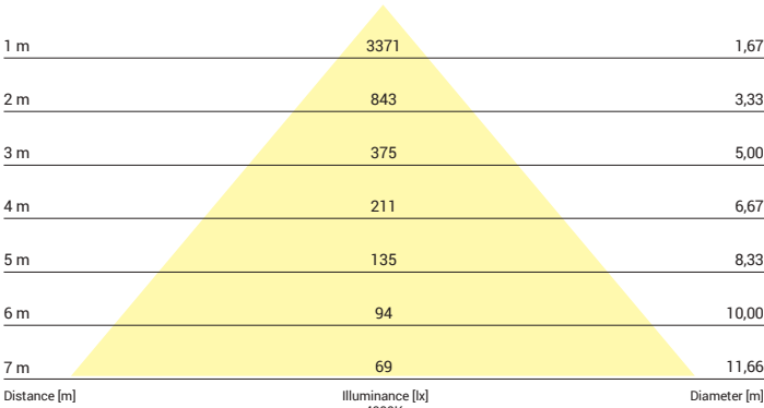
8260, 40W, 4000K, beam angle 80°
