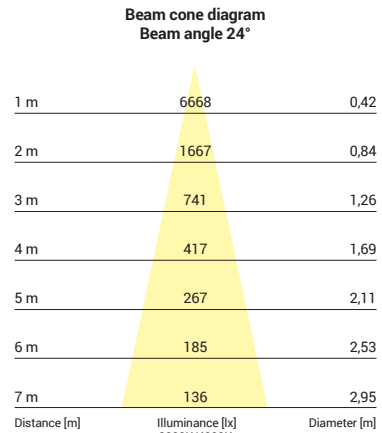
8763, 8764, 8765, 8766, 15W, 3000K, 4000K, beam angle 24°
