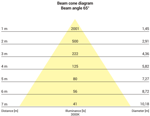
8768, 40W, 3000K, beam angle 65°
