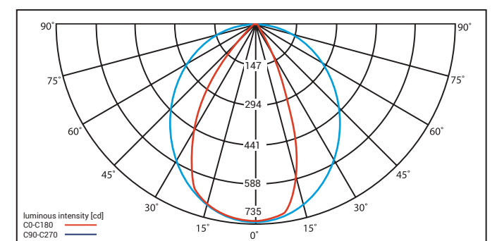
Beam cone diagram - 8452 BL
